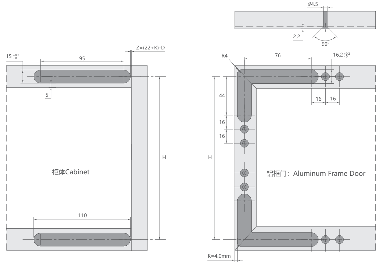
装底盒柜体开孔尺寸 Dimensions of cabinet bottom drilling
