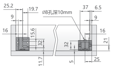
铁尾支架 Metal Rear Bracket 塑胶尾支架 Plastic Rear Bracket
